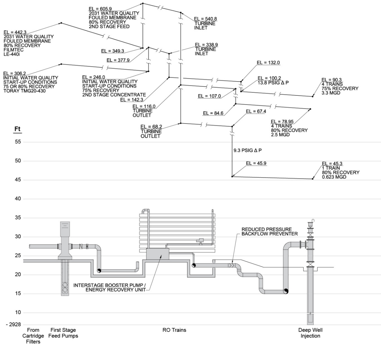
Figure 3-4. Sample hydraulic profile – membrane concentrate.
