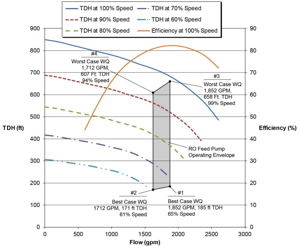
Figure 4-9. Reverse osmosis feed pump operating envelope.
