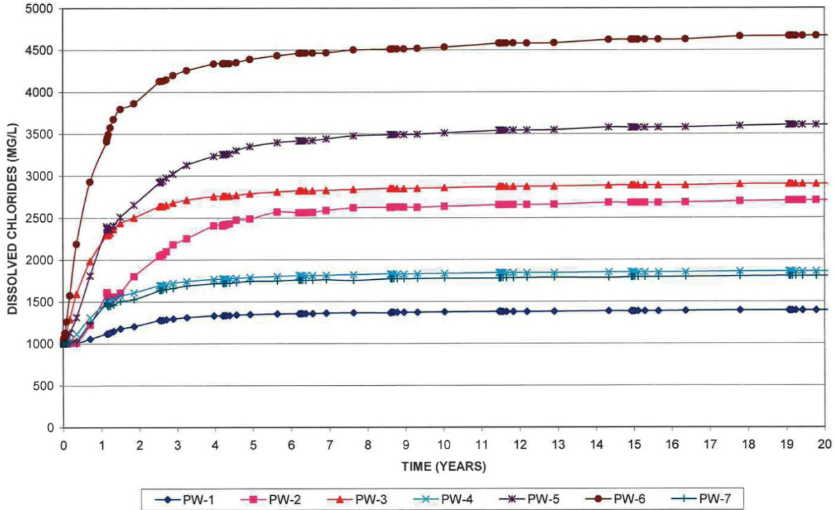
Figure 3-1. Projected dissolved chloride variations at brackish well field.
