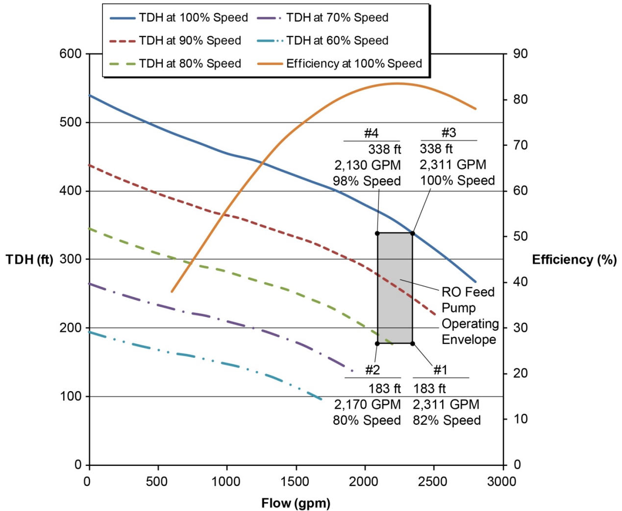
Figure 4-4. Example 1 - reverse osmosis feed pump operating envelope.
