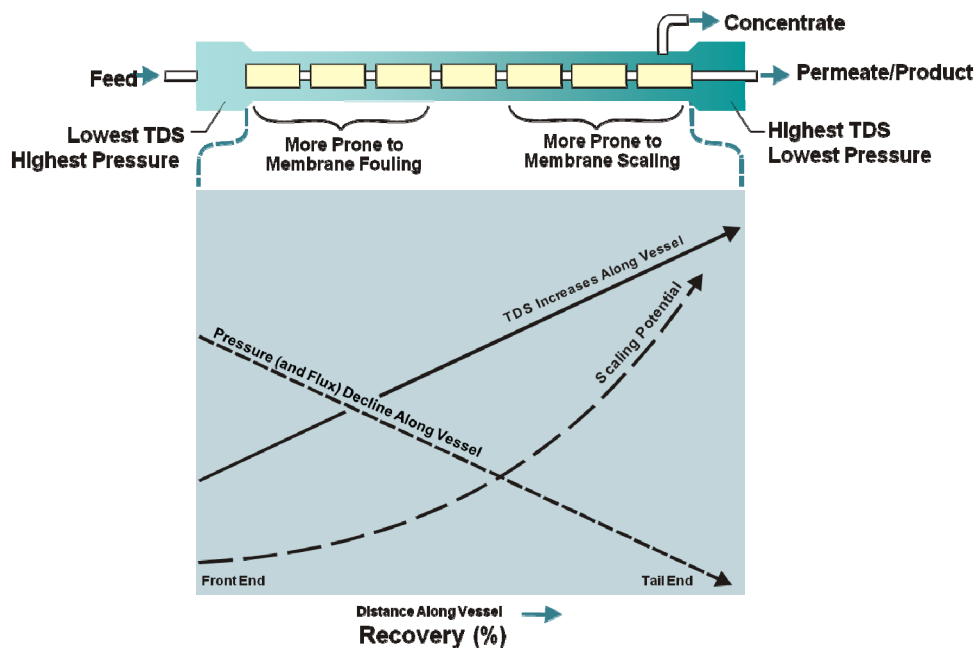
Figure 3-5. Flux decline within a pressure vessel.
