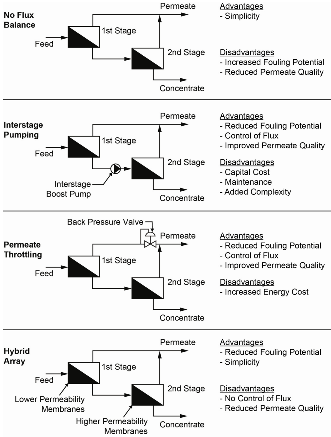
Figure 3-6. Flux balancing alternatives.
