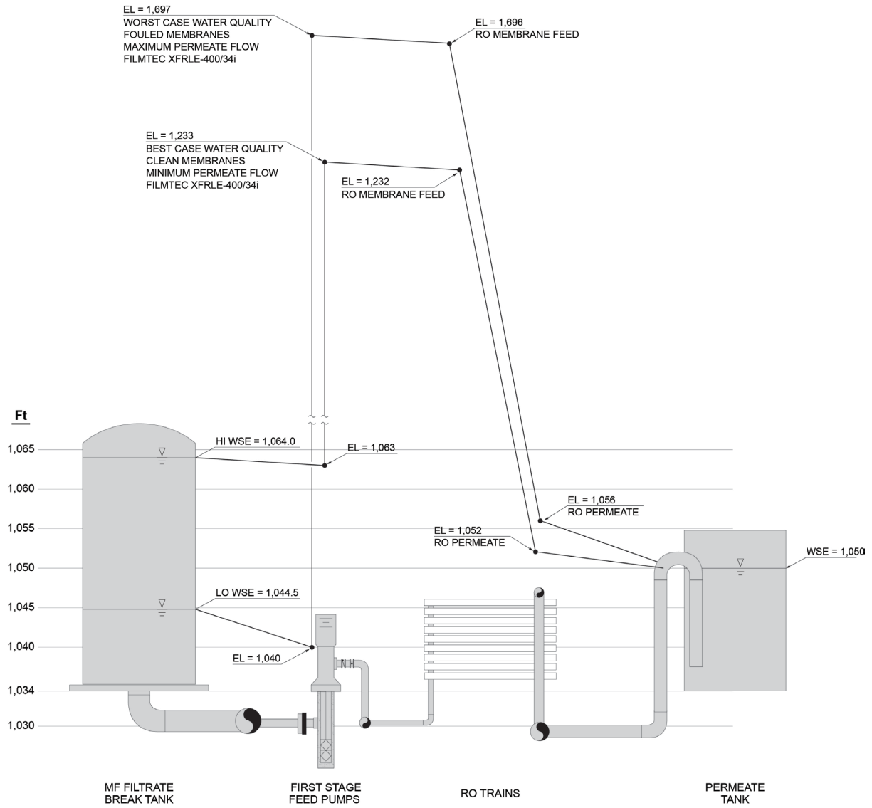
Figure 4-8. Example 2 hydraulic profile.
