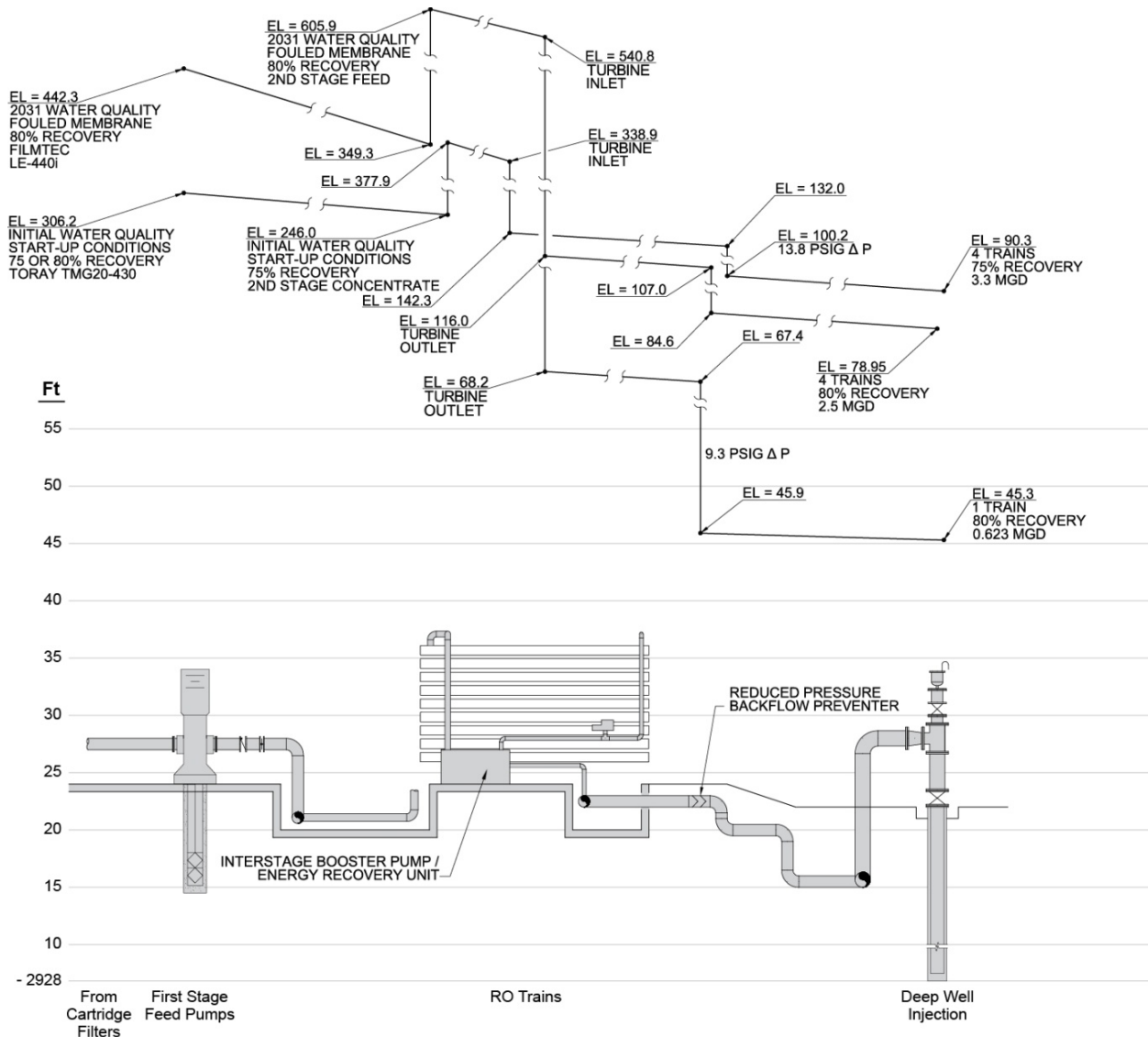
Figure 4-5. Example 1 hydraulic profile - membrane concentrate.
