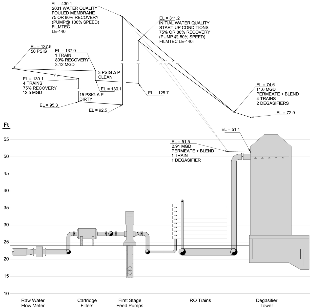
Figure 4-3. Example 1 hydraulic profile – membrane feed and permeate.
