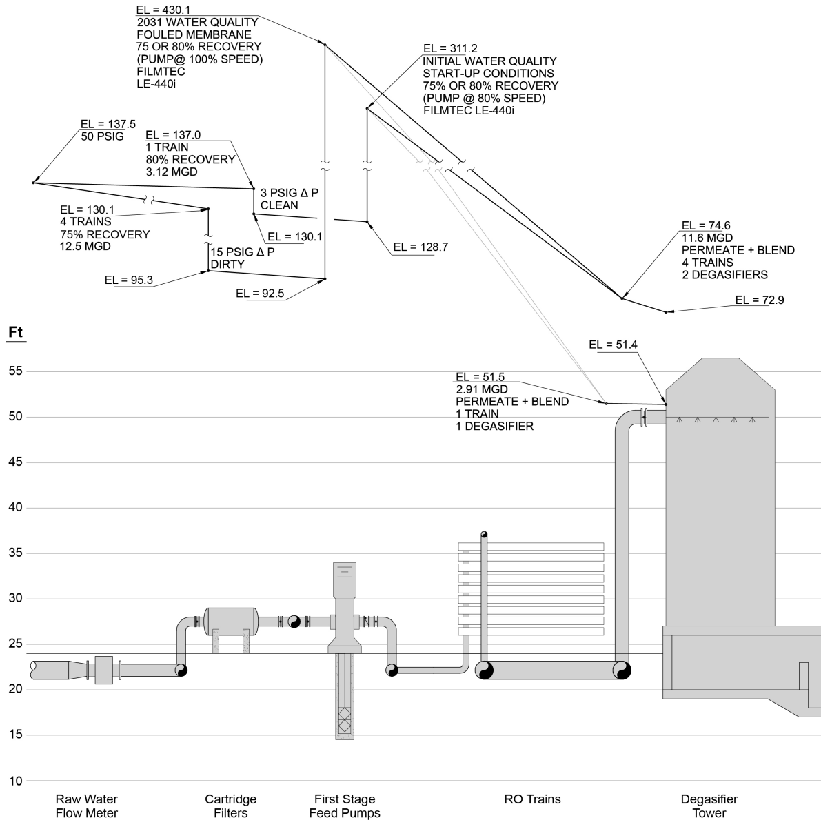
Figure 3-3. Sample hydraulic profile – membrane feed and permeate.
